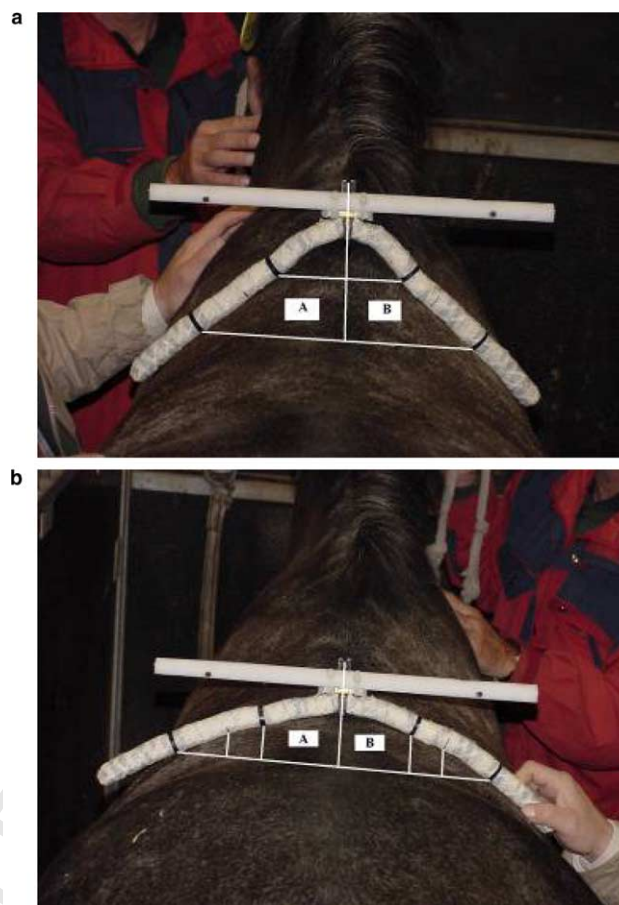
Fig. 2. Back gauge, used for taking measurements at the withers (a) and in the thoracolumbar area (b).
